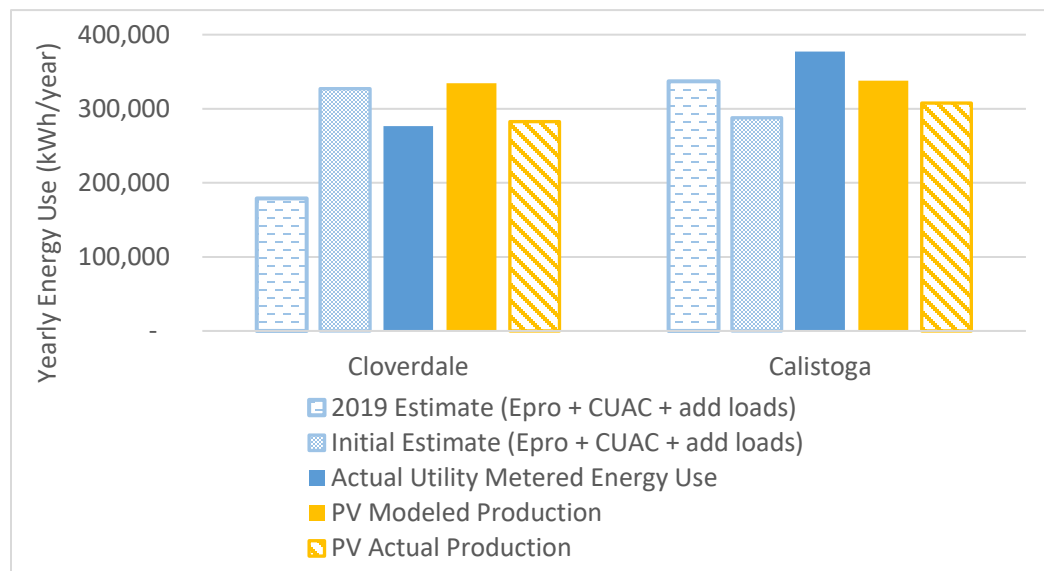
Figure 1: Calistoga and Cloverdale modeled whole site energy use and solar PV production compared to 2019 actual utility-monitored energy use.
