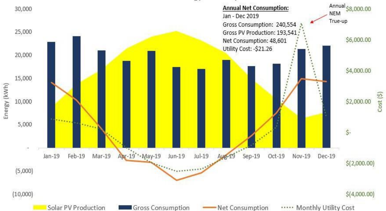
Edwina Benner Plaza: Common Area Energy Consumption and Solar PV Production
