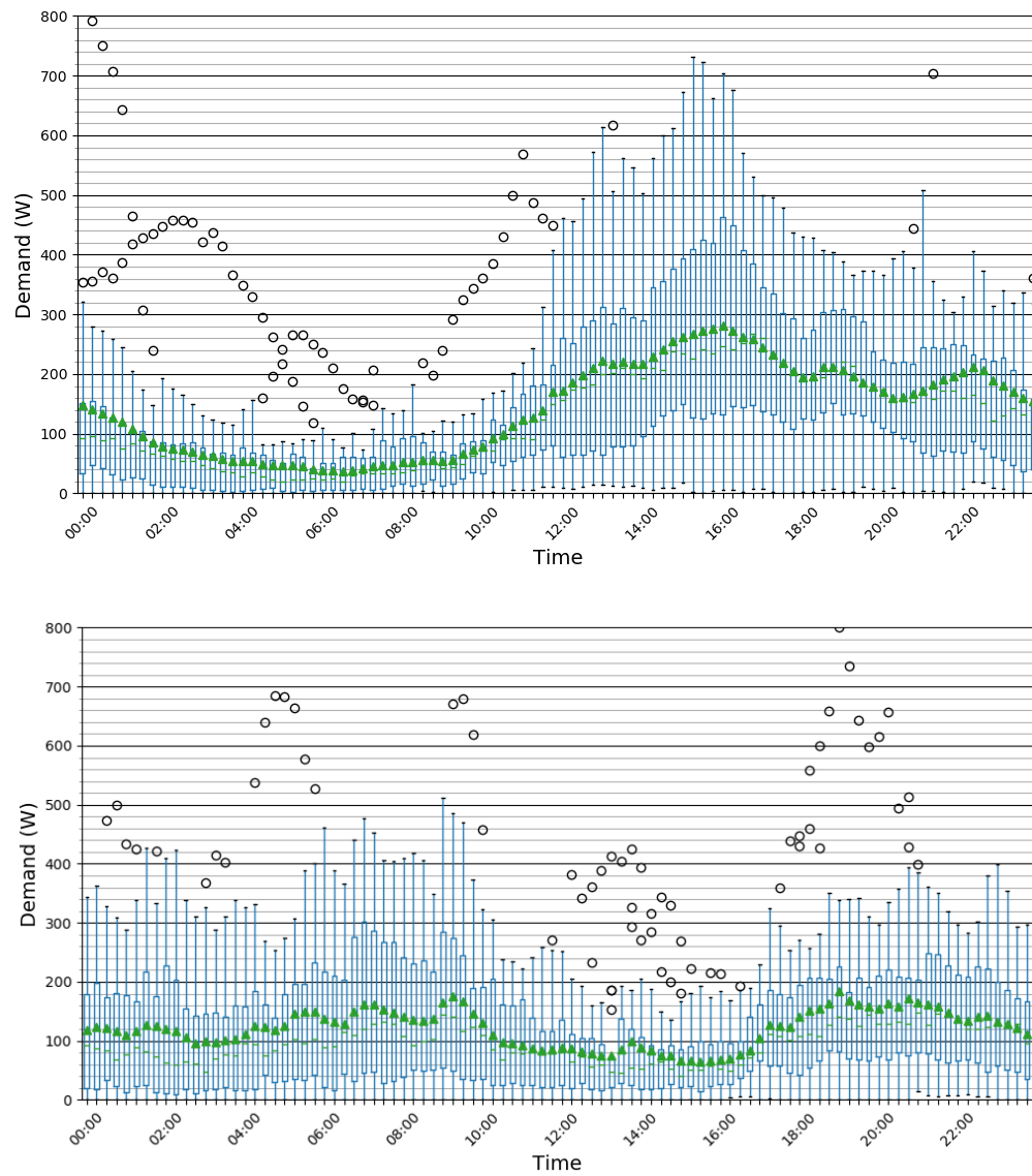
Figure E-30: Seasonal demand by summer (top), winter (middle) and shoulder (bottom) seasons
