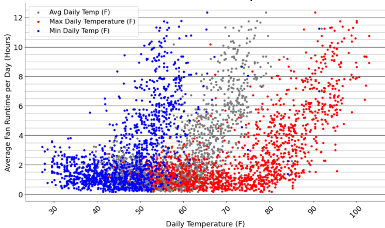
Figure D-11: Fan Coil Runtime for Both Sites Shows Little Sensitivity to Cooler Outdoor Ambient Temperatures
